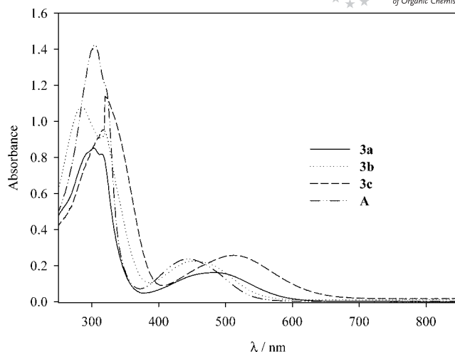
Figure 2. Absorption spectra of TTF derivatives 3a–c in CH 2 Cl 2 /CH 3 CN ( c = 5 \times 10^{-5} \text{ mol L}^{-1} ).
