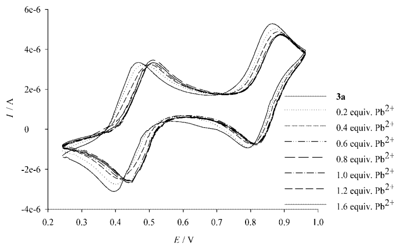
Figure 5. CV titration of compound 3a ( c = 7.5 \times 10^{-4} \text{ mol L}^{-1} ) in \text{CH}_2\text{Cl}_2/\text{CH}_3\text{CN} (1:1, v/v) in the presence of increasing amounts of lead perchlorate [ 70 \text{ mV s}^{-1} , \text{NBu}_4\text{BF}_4 ( c = 10^{-1} \text{ mol L}^{-1} ), vs. \text{Ag}/\text{AgCl} ].
