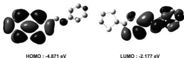
Figure 1. Frontier orbitals of 3a calculated by DFT at the B3LYP/6-31G(d,p) level of theory.
