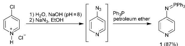
Scheme 1. Synthesis of the iminophosphorane 1 .
