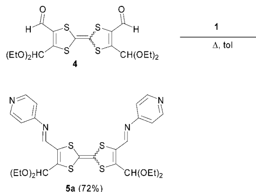
Scheme 2. Synthesis of the conjugated TTF-imine systems.
