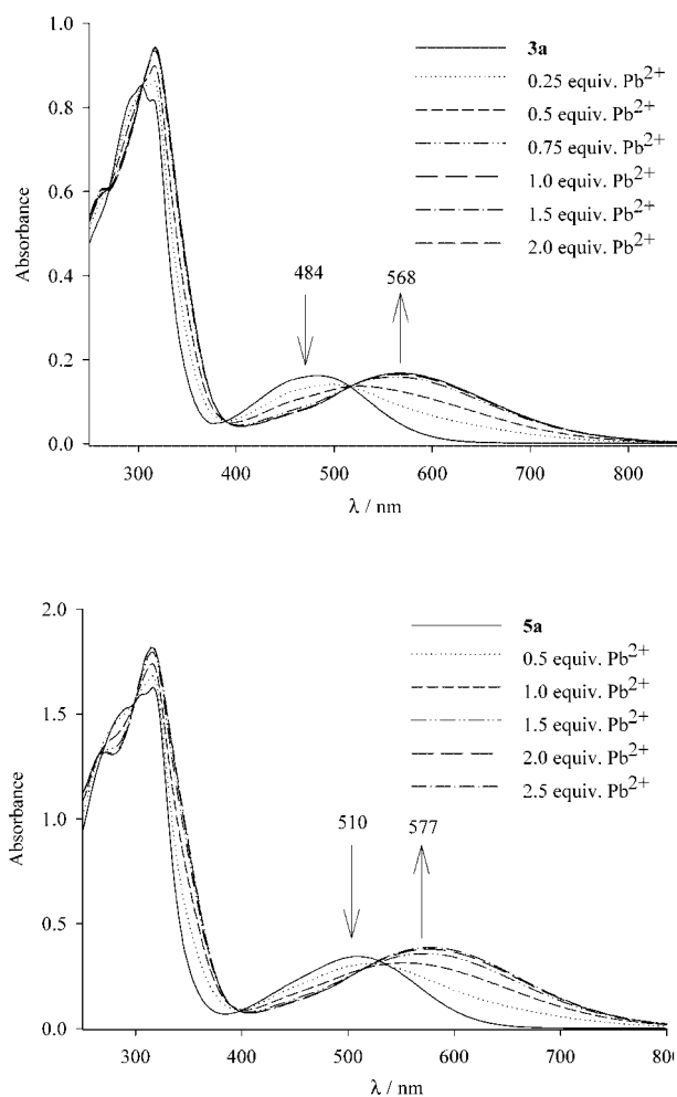
Figure 3. UV/Vis titration study of 3a (top) and 5a (bottom) [ c = 5 \times 10^{-5} \text{ mol L}^{-1} in \text{CH}_2\text{Cl}_2/\text{CH}_3\text{CN} (1:1, v/v)] in the presence of \text{Pb}(\text{ClO}_4)_2 .
