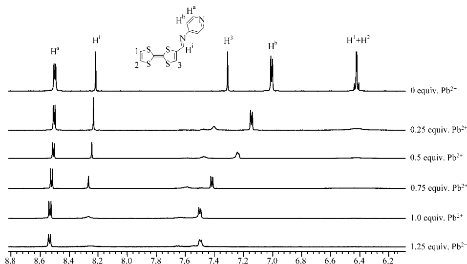
Figure 4. 1 H NMR spectra of 3a ( c = 9.5 \times 10^{-3} \text{ mol L}^{-1} ) in \text{CD}_3\text{CN}/\text{CD}_2\text{Cl}_2 (1:1, v/v) in the presence of increasing amounts of \text{Pb}(\text{ClO}_4)_2 .
